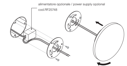
cassaforma a filo parete flush with the installation surface cassaforma / installation box cod. F1318000
