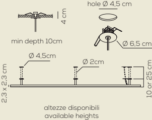
rosone incasso / recessed canopy
