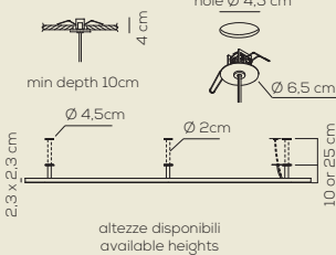
rosone incasso / recessed canopy hole Ø 4.5 cm
